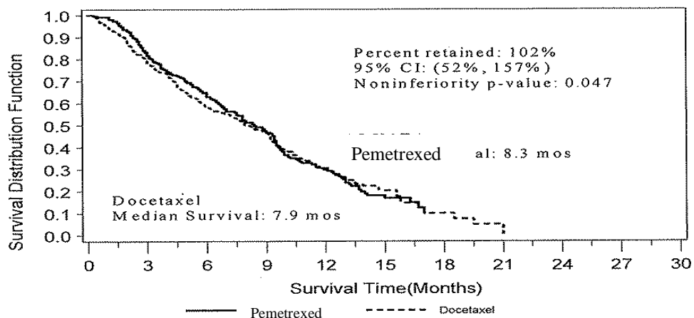
Figure 10: Kaplan-Meier Estimates of Survival Time for Pemetrexed versus Docetaxel
