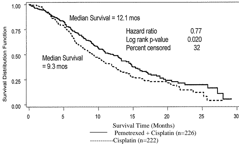
Figure 1: Kaplan-Meier Estimates of Survival Time
